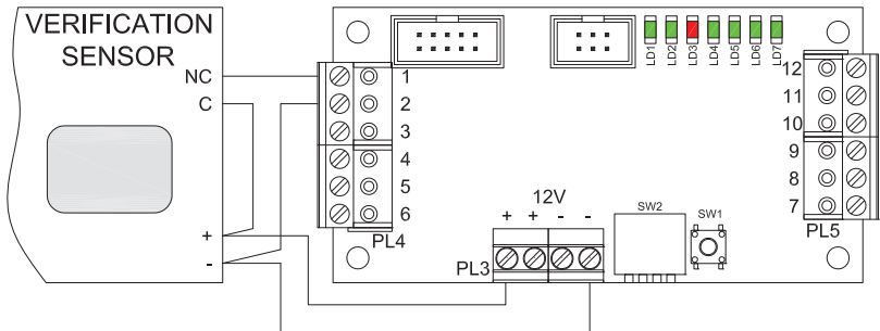
SmokeCloak Easy interface to alarm panel wiring VERIFICATION SENSOR CONNECTION 3257-A
